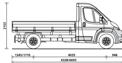
Platforma s kabinom L3/L4
