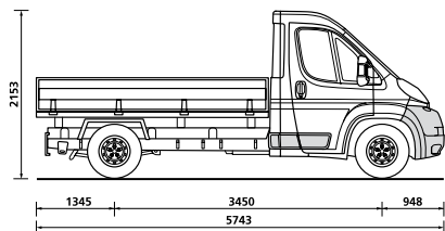
Platforma s kabinom L2
